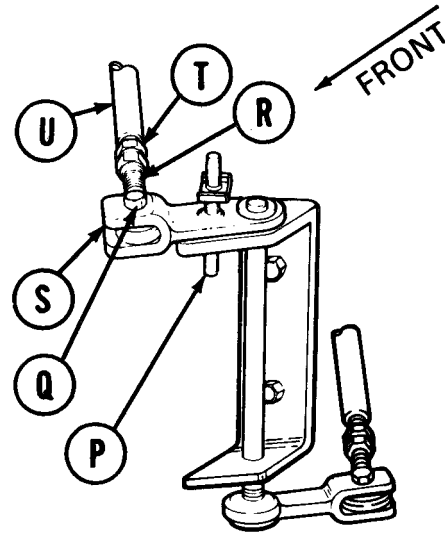
DRIVER'S STATION
