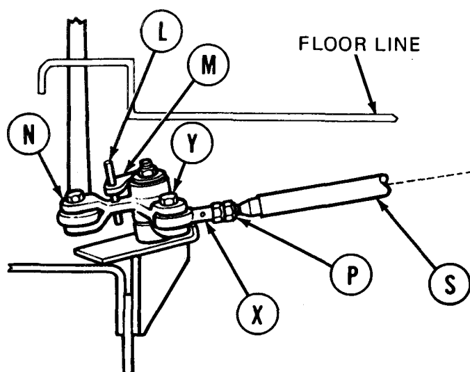
FORWARD INBOARD LINK ASSEMBLY
