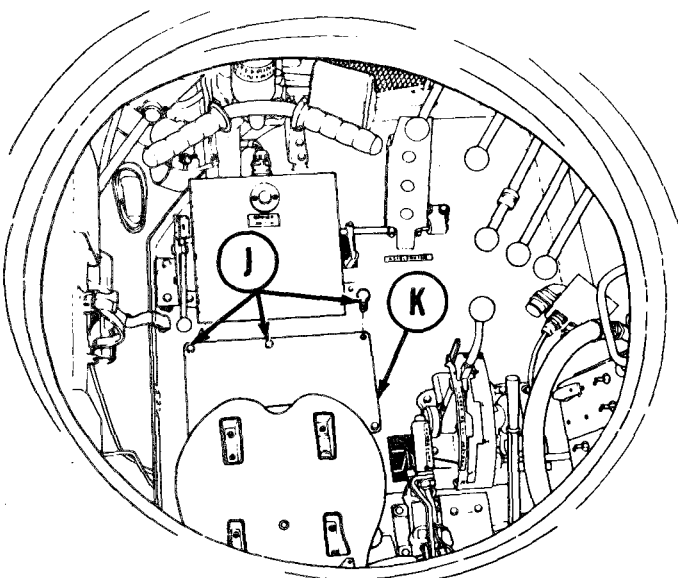
DRIVER'S STATION
