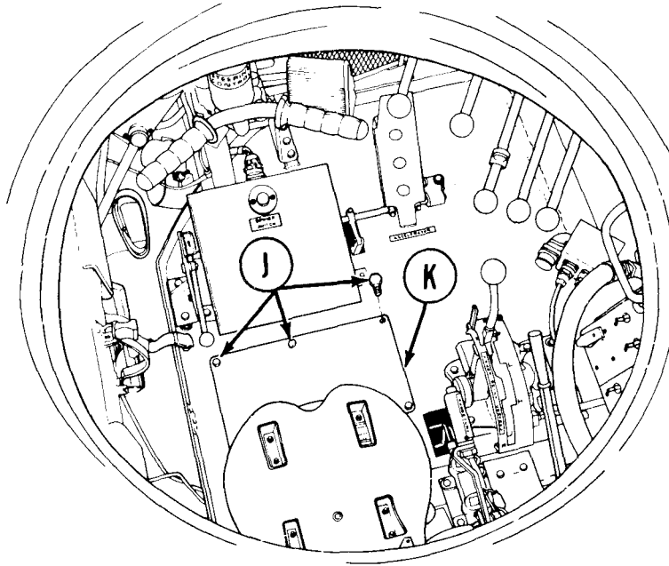
DRIVER'S STATION
